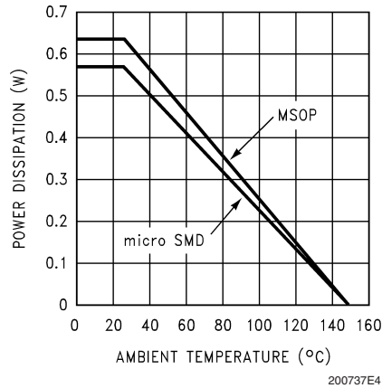
Power Derating Curve
