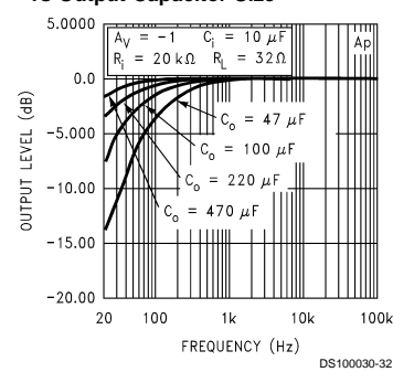
Frequency Response vs Output Capacitor Size
