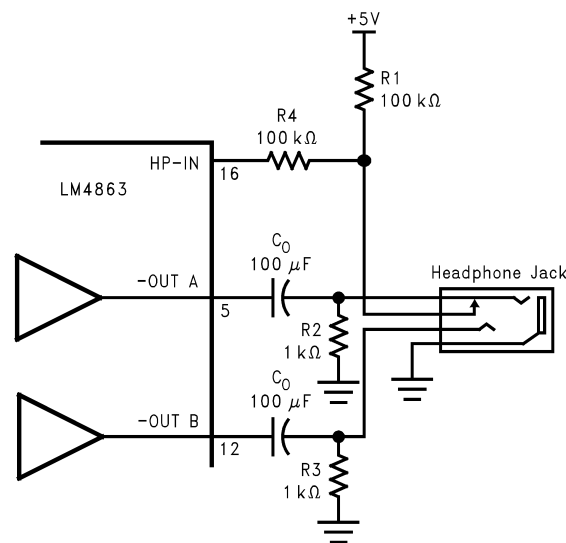
FIGURE 3. Headphone Circuit
