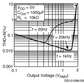
THD+N vs Output Voltage Docking Station Pins
