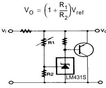
Figure 15. High Current Shunt Regulator
