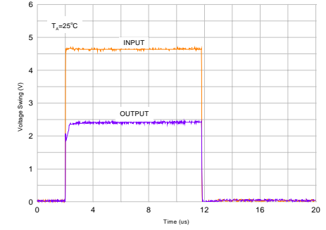
Figure 9. Pulse Response
