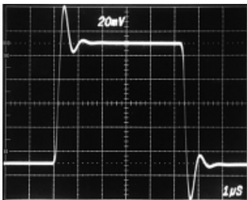
TA=225°C, CL=100pF
