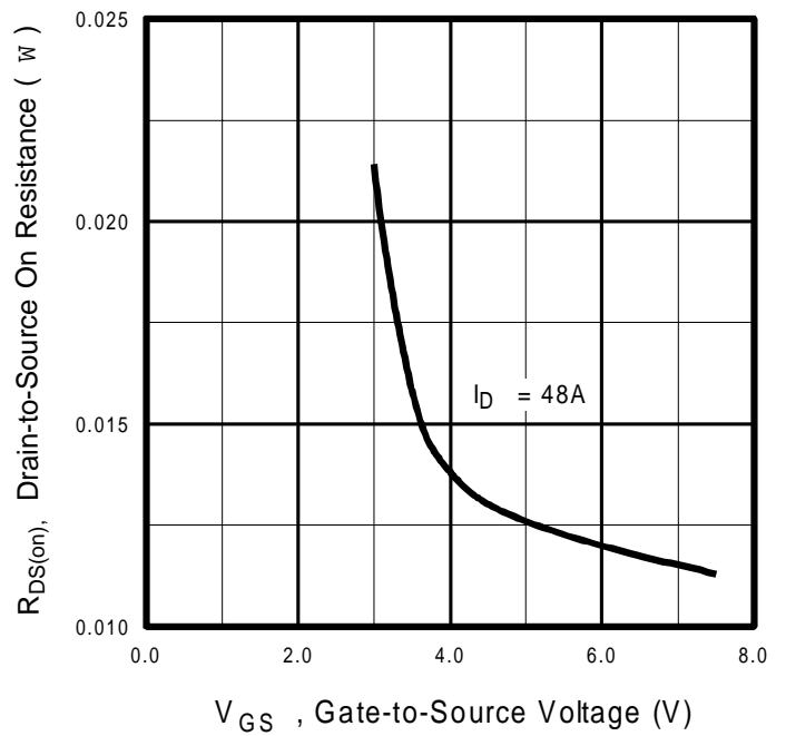
Fig 13. On-Resistance Vs. Gate Voltage
