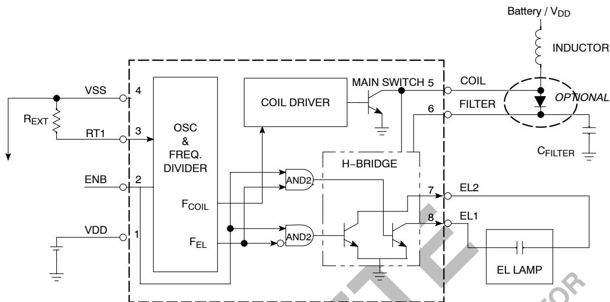
Figure 1. Test Circuit
