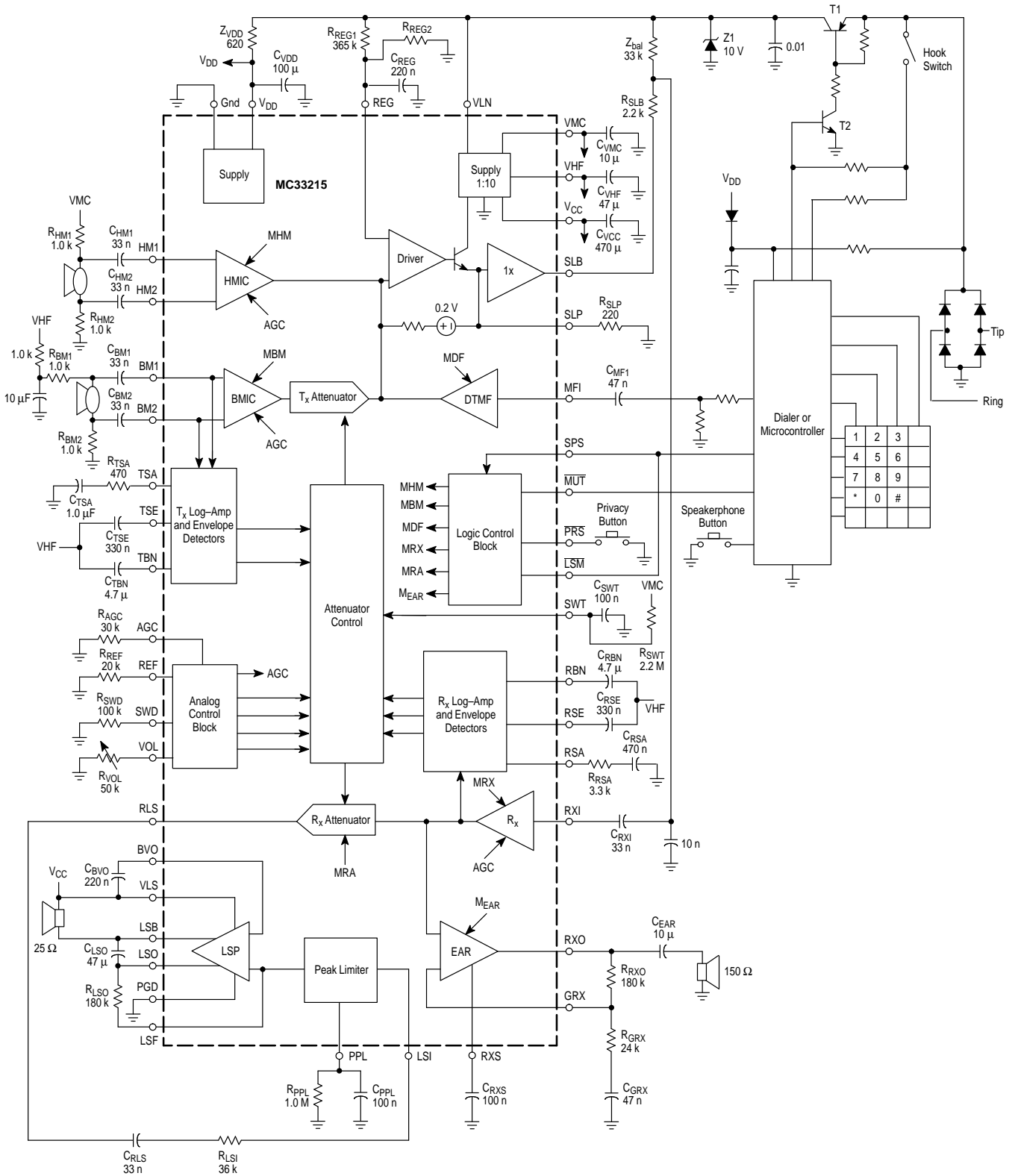
Figure 18. Typical Application
