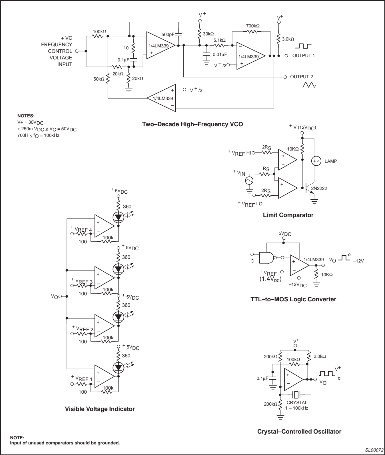
Figure 3. Equivalent Circuit
