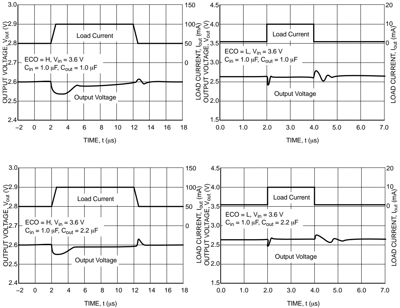
Figure 30. Load Transient Response (V out = 2.6 V)
