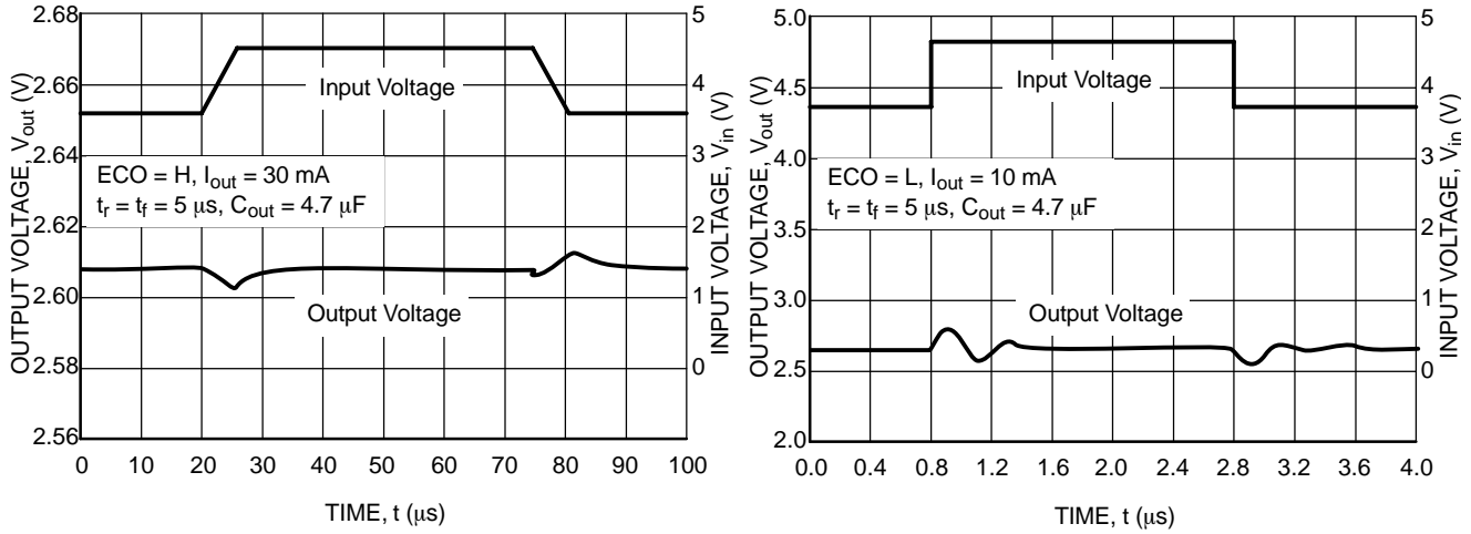
Figure 29. (continued) Input Transient Response (V out = 2.6 V)
