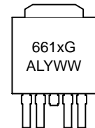
DPAK-5 CENTER LEAD CROP CASE 175AA
