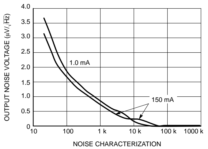
Figure 7. Output Noise Voltage
