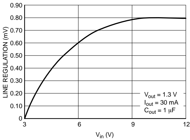
Figure 10. Line Regulation
