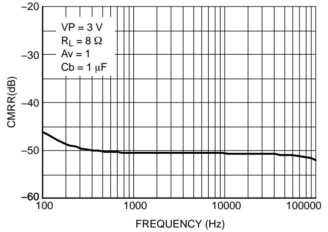
Figure 16. CMRR @ V_P = 3 \text{ V}
