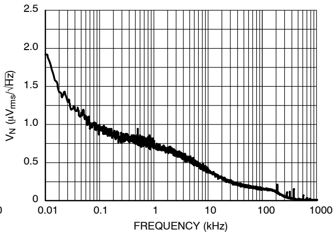
Figure 32. Output Voltage Noise, 2.5 V Version, V_{IN} = 3.5 V
