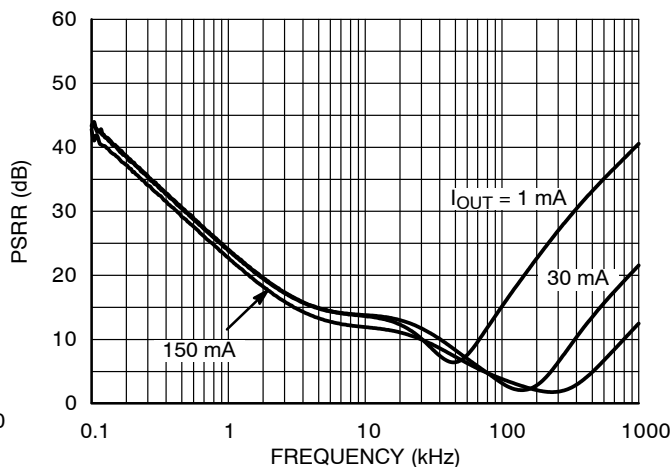
Figure 28. PSRR, 2.5 V Version, V_{IN} = 3.5 V
