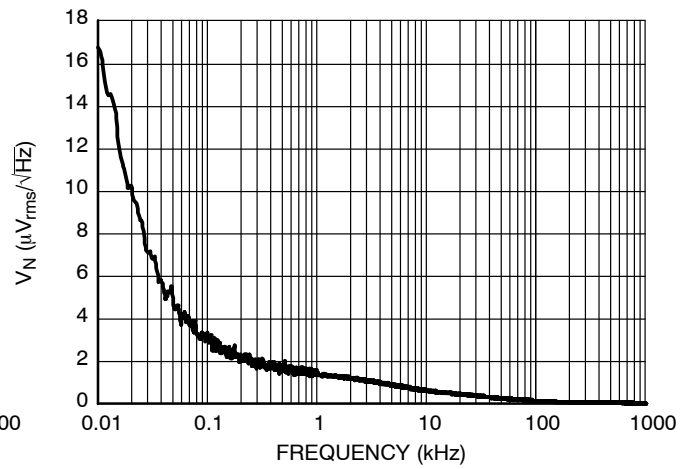
Figure 34. Output Voltage Noise, 3.3 V Version, V_{IN} = 4.3\text{ V}
