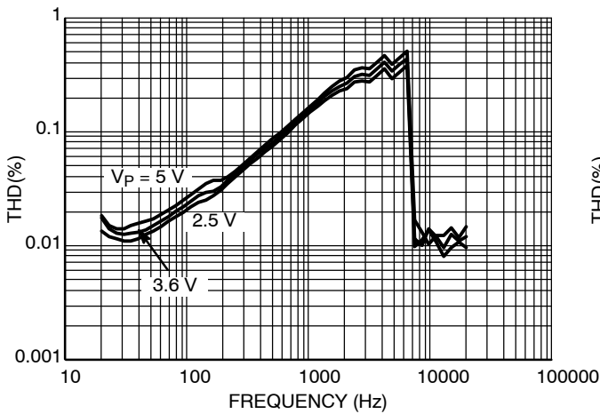
Figure 7. THD+N vs Frequency P out = 250 mW, R L = 8 Ω
