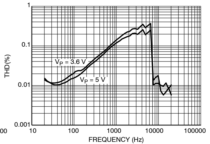
Figure 8. THD+N vs Frequency P out = 500 mW, R L = 8 Ω
