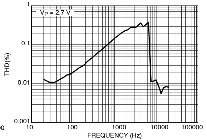
Figure 6. THD+N vs Frequency P out = 150 mW, R L = 8 Ω
