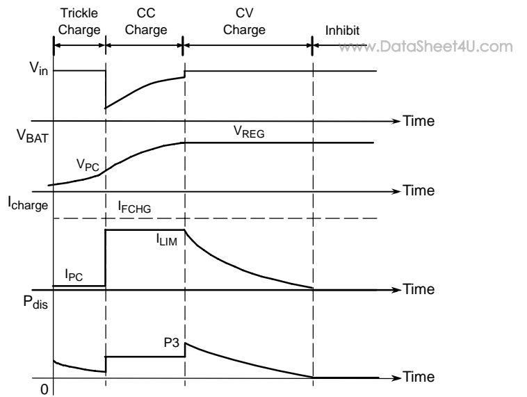
Figure 17. Typical Charge Curves with a Current Limited Adapter
