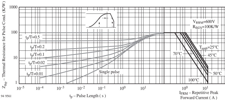
Figure 7. Thermal Response
