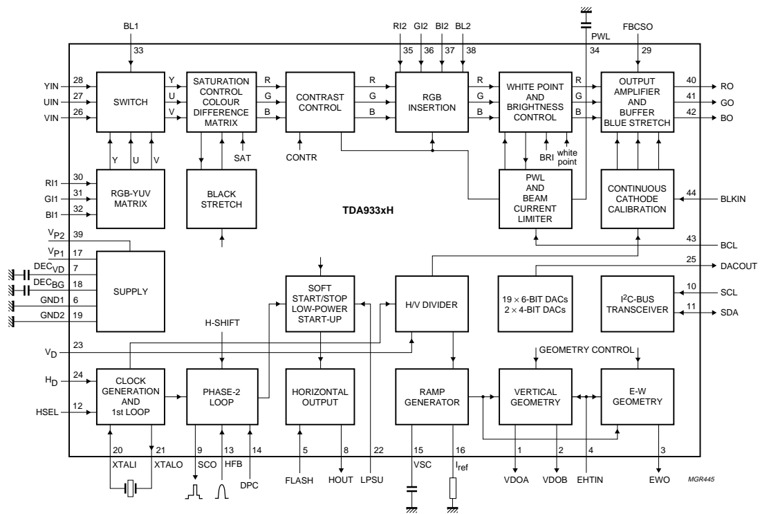
Fig.1 Block diagram.
