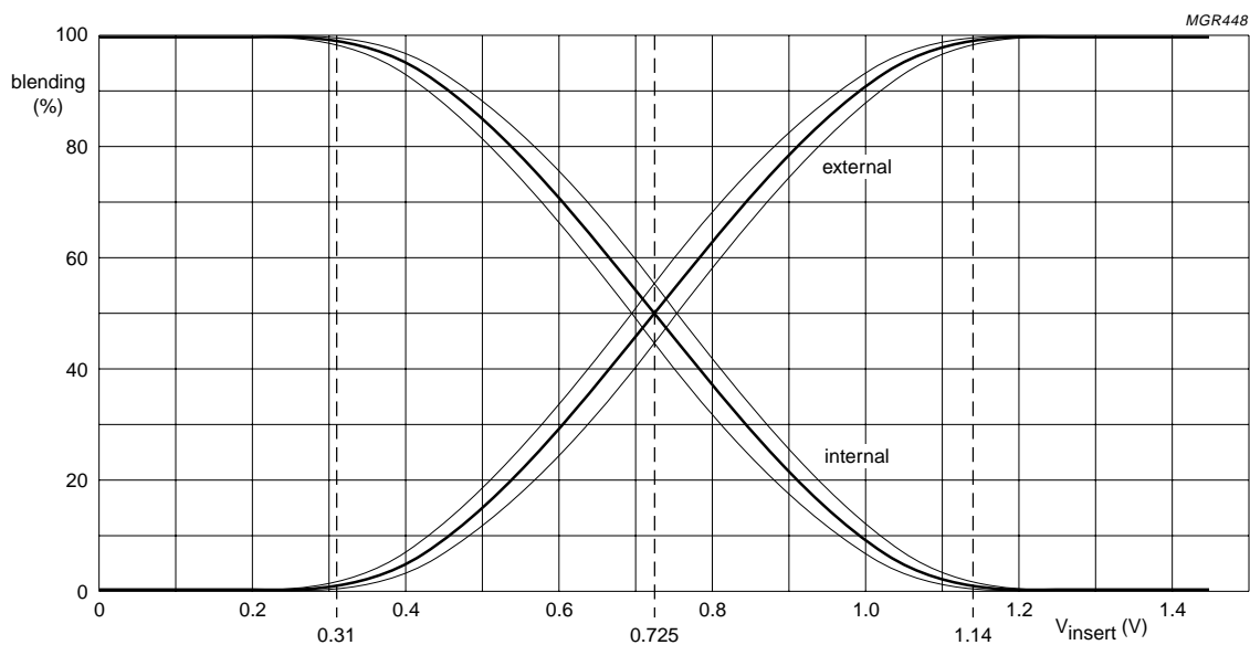
Fig.4 Blending characteristic (typical curve and minimum/maximum limits).
