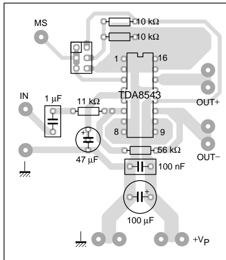
b. Component side.
