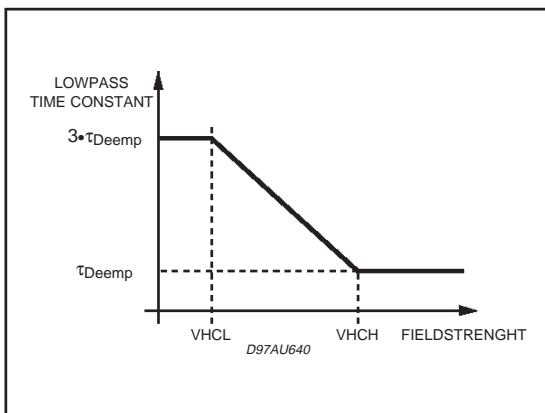
Figure 16. Highcut Characteristics
