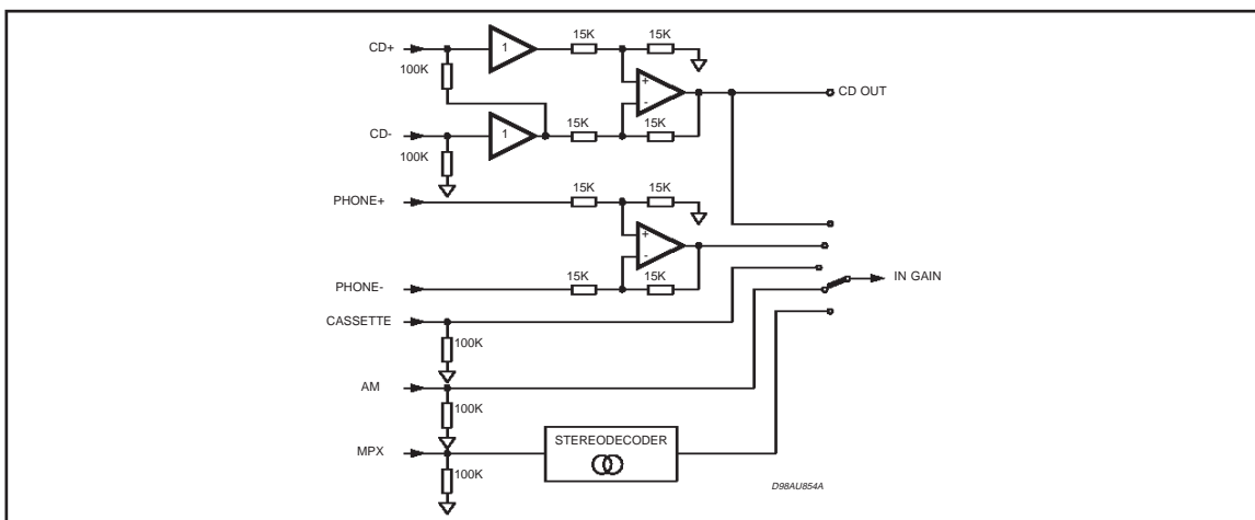
Figure 4. Input stages
