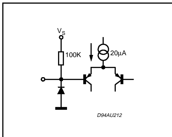
PIN: ADDR
