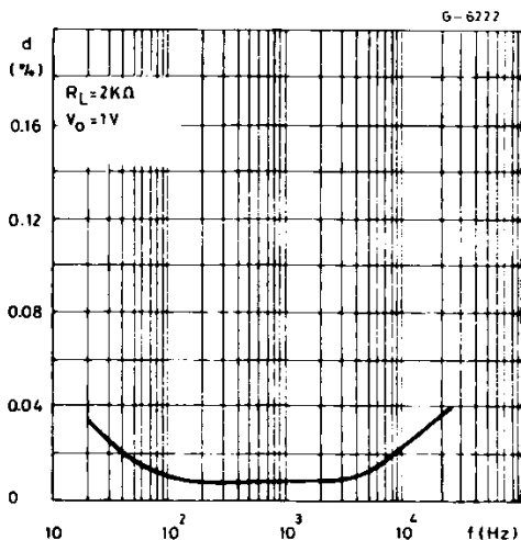
Figure 11 : Distortion vs. Frequency (compressor).
