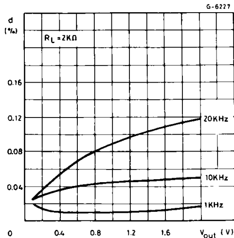
Figure 15 : Distortion vs. Output Voltage (op. amp. 2).
