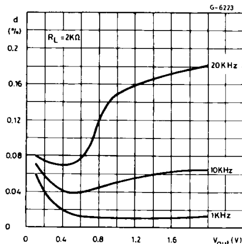
Figure 12 : Distortion vs. Output Voltage (op. amp. 1 & 3).
