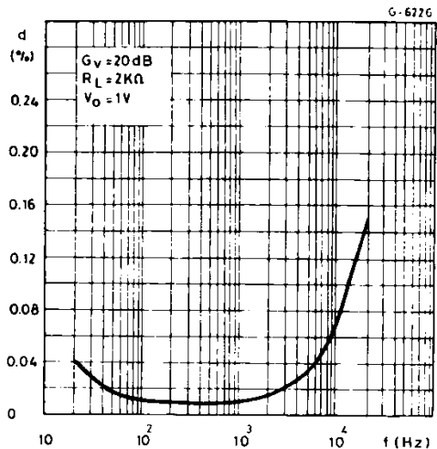
Figure 13 : Distortion vs. Frequency (op. amp. 1 & 3).
