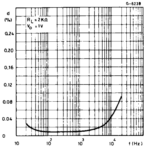
Figure 16 : Distortion vs. Frequency (op. amp. 2).
