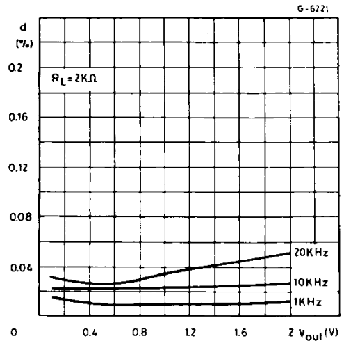
Figure 8 : Distortion vs. Output Voltage (input differ. amplifier).
