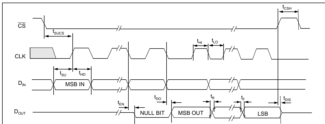
FIGURE 1-1: Serial Timing.
