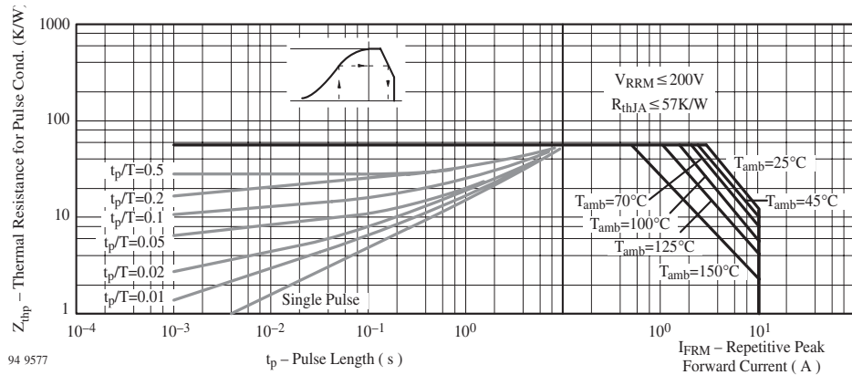
Figure 7. Thermal Response
