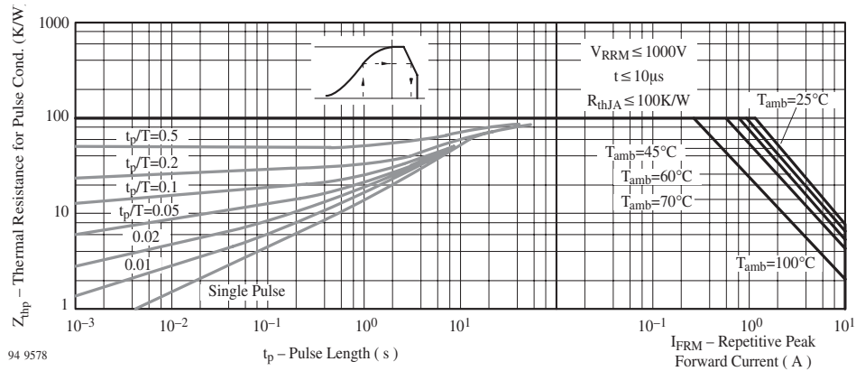
Figure 6. Thermal Response
