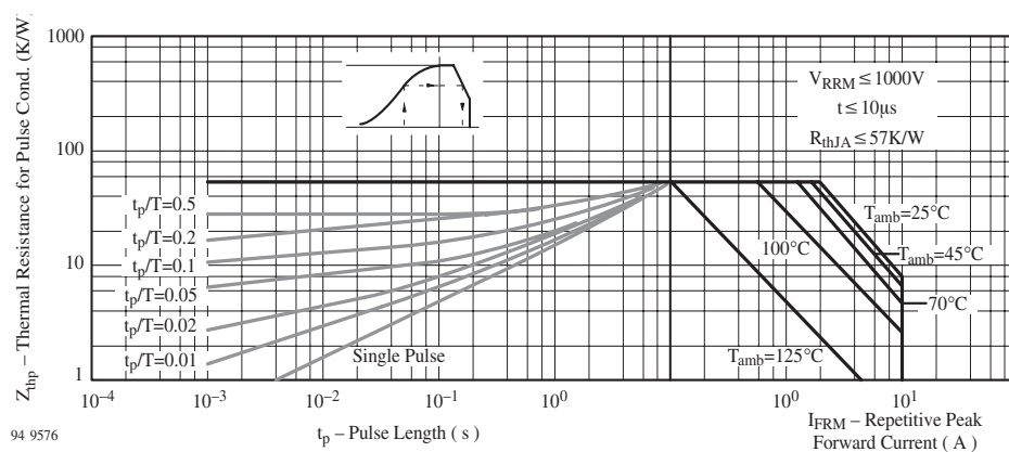
Figure 8. Thermal Response
