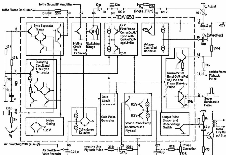
TDA1950 Application Circuit and Block Diagram
