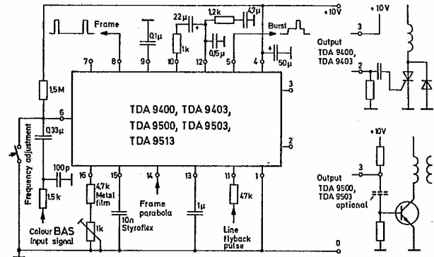
Application Circuit
