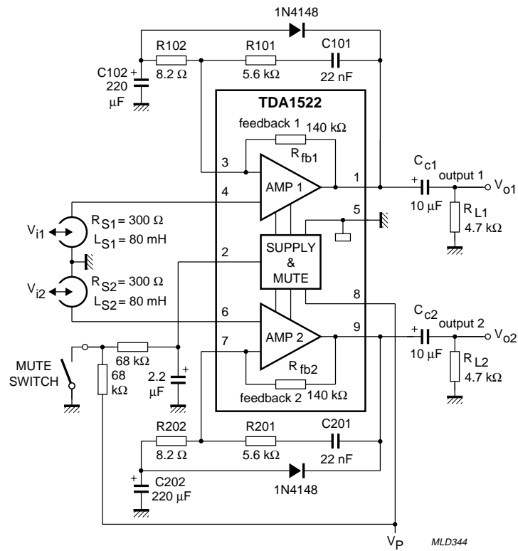
Fig.10 Application for pop-free muting.
