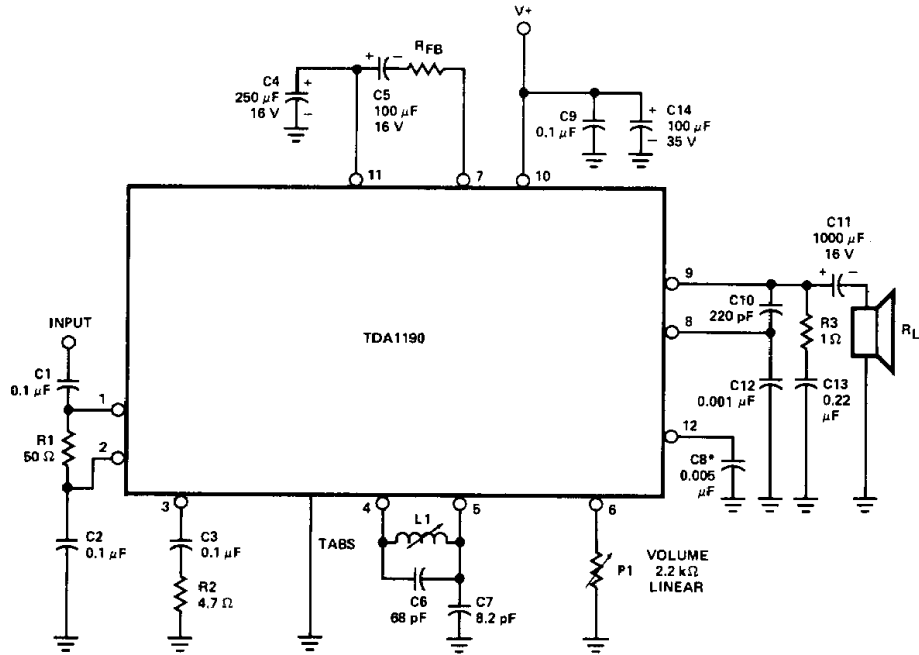
TEST CIRCUIT – TDA1190
