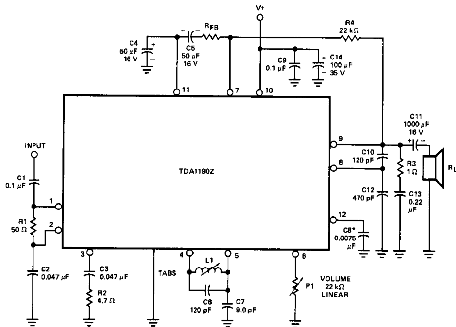
TEST CIRCUIT – TDA1190Z
