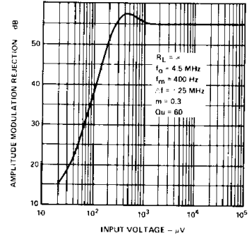
AMR AS A FUNCTION OF INPUT VOLTAGE
