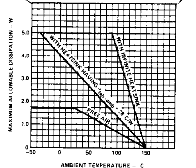
MAXIMUM ALLOWABLE DISSIPATION AS A FUNCTION OF AMBIENT TEMPERATURE
