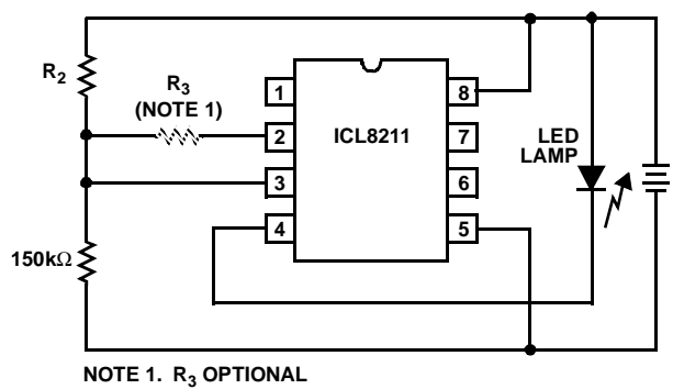
NOTE 1. R 3 OPTIONAL FIGURE 28. LOW VOLTAGE BATTERY INDICATOR
