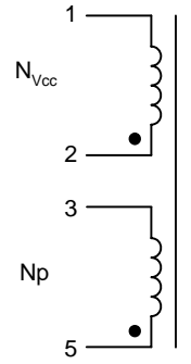
Figure 38. Inductor Schematic Diagram
