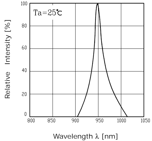
Fig. 4 Spectrum Distribution
