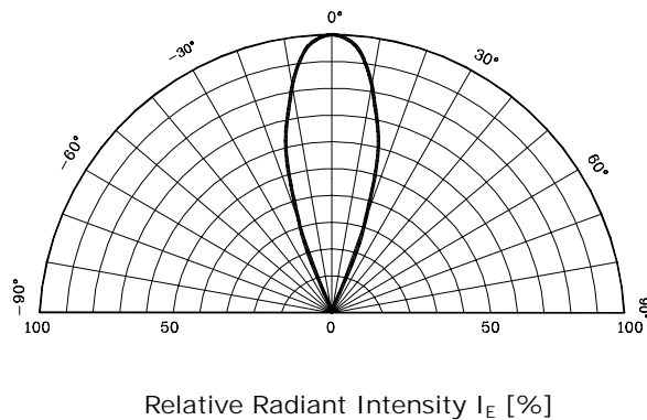
Fig. 5 Radiation Diagram
