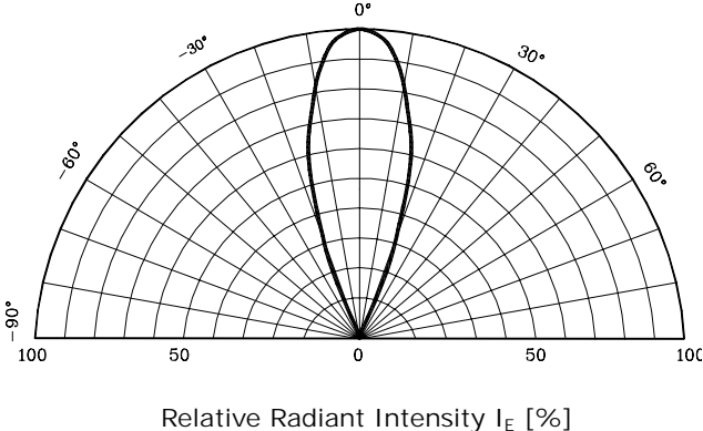
Fig. 5 Radiation Diagram
