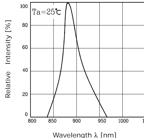
Fig.4 Spectrum Distribution
