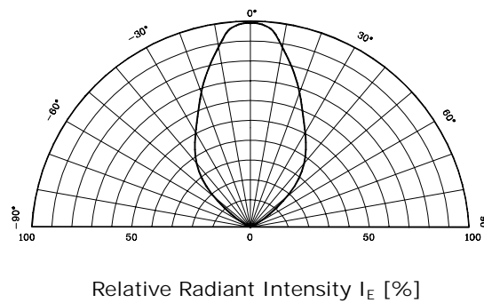
Fig. 5 Radiation Diagram
