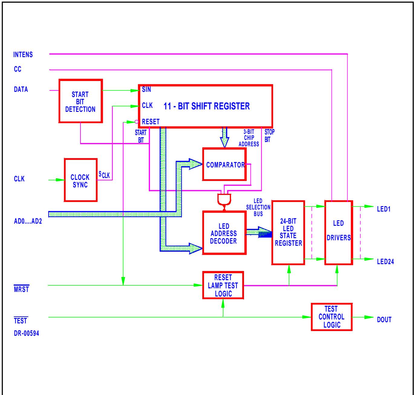
FIGURE 1: BLOCK DIAGRAM
