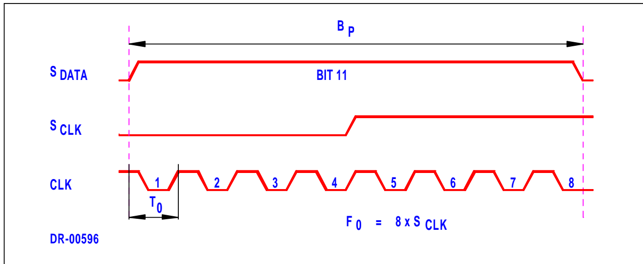
FIGURE 3: TIMING DIAGRAM
