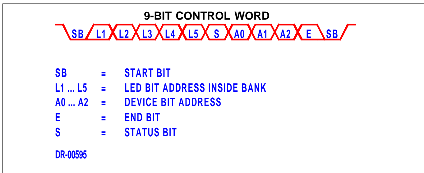
FIGURE 2: CONTROL WORD STRUCTURE
