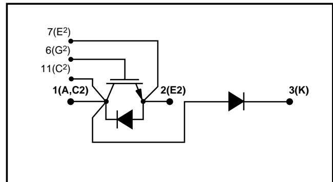
Fig. 1 Chopper circuit diagram - lower arm controlled
