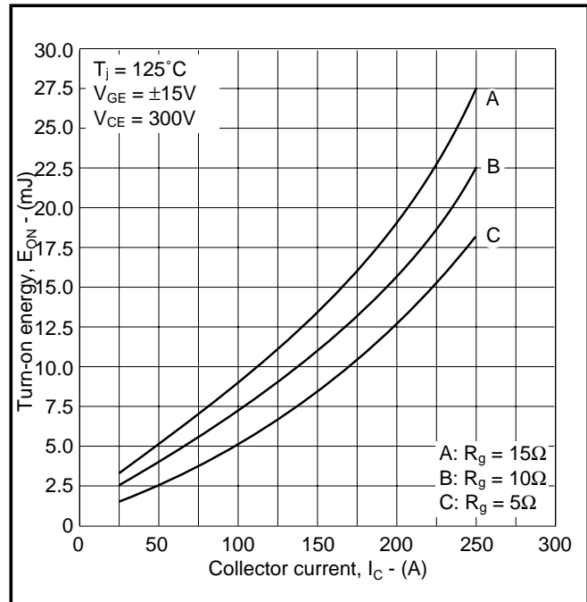
Fig.6 Typical turn-on energy vs collector current
