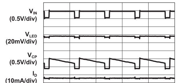
Line Response (1.5X Mode, 3x30mA Load)
