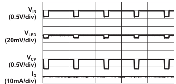
Line Response (1X Mode, 3x30mA Load)
