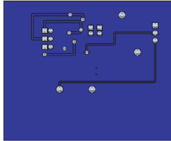
Figure 4: AAT3128 Evaluation Board Solder Side PCB Layout.
