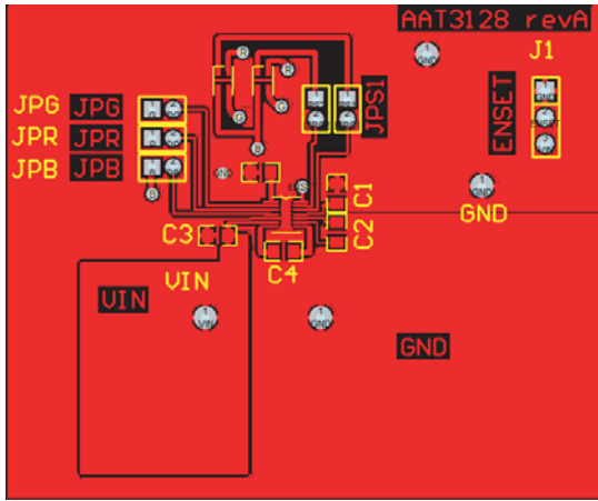
Figure 3: AAT3128 Evaluation Board Component Side PCB Layout.
