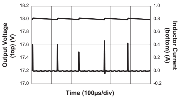
Output Ripple ( V_{IN} = 4.2V ; V_{OUT} = 18V ; No Load)
