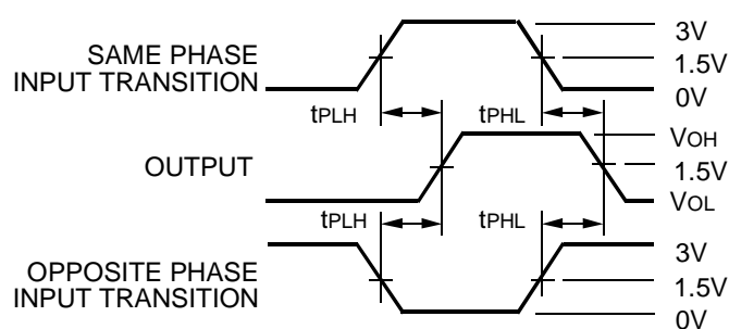
Propagation Delay
