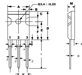
TO-247 (3P)
