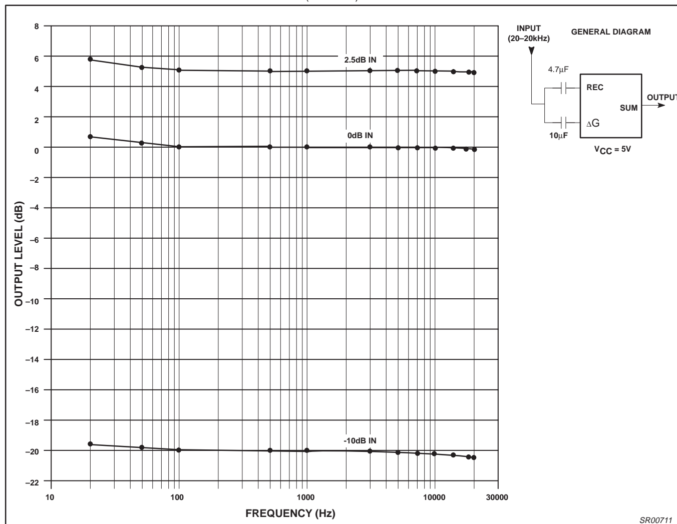
Figure 9. Expander Output Frequency Response
