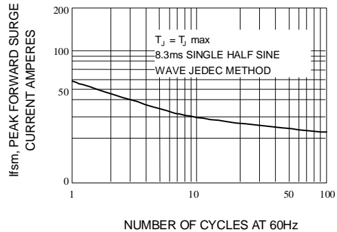
Fig. 6-MAXIMUM NON-REPETITIVE PEAK FORWARD SURGE CURRENT UNIDIRECTIONAL ONLY
