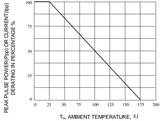
Fig. 2-PULSE DERATING CURVE
