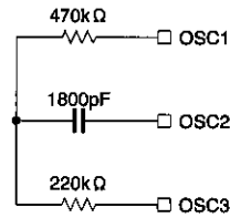
Oscillator circuit 1
