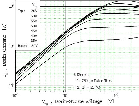
Fig 1. Output Characteristics
