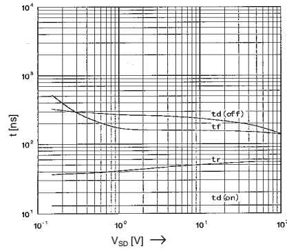
Typical Switching Characteristics
