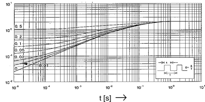
Transient Thermal impedance
