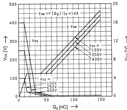
Typical Input Charge
