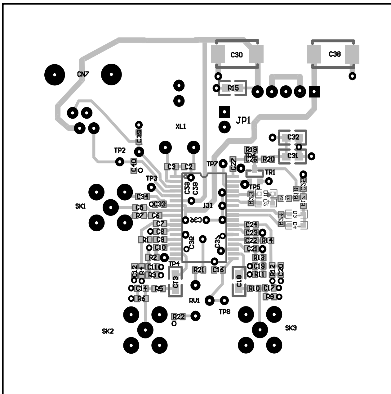
Figure 20. Bottom view
