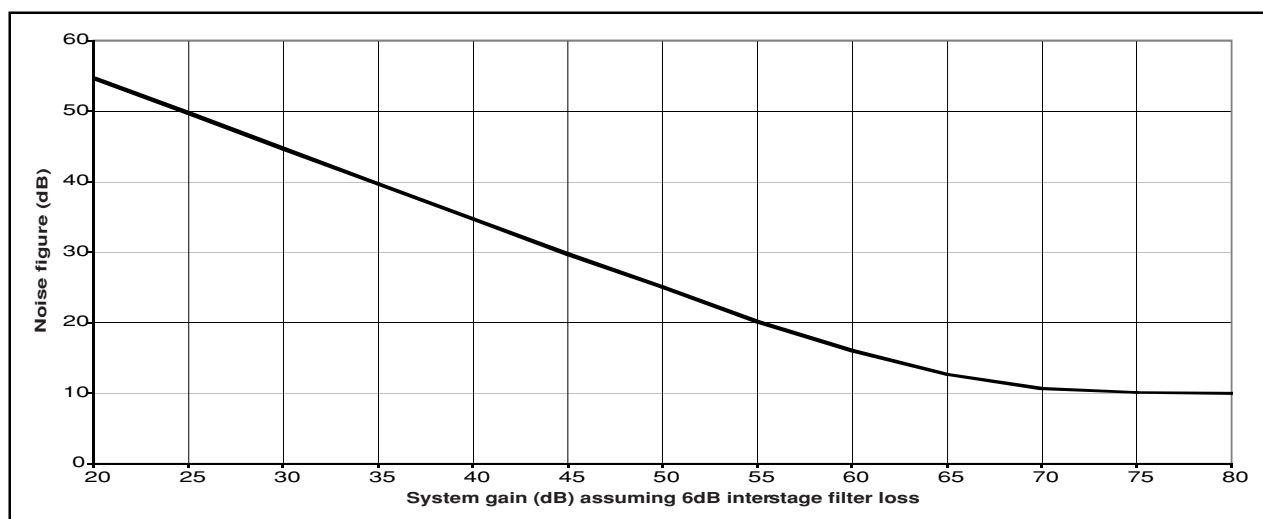
Figure 8. Variation in NF with system gain (typical)
