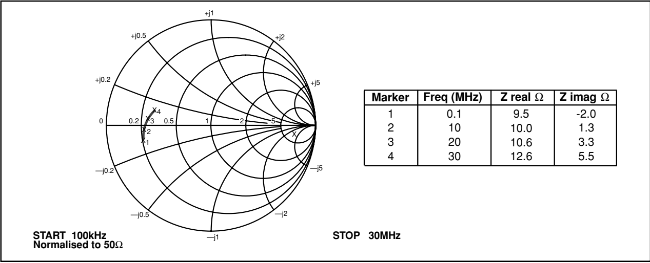
Figure 12. Baseband output impedance; IOU, QOUT (typical)
