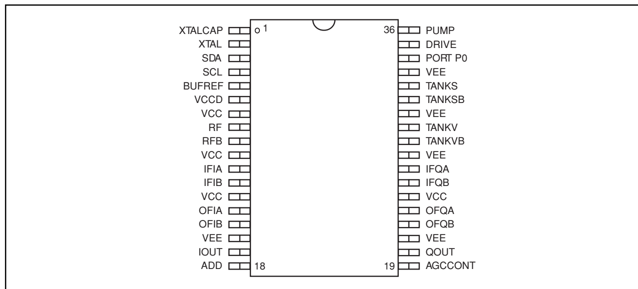
Figure1. Pin connections
