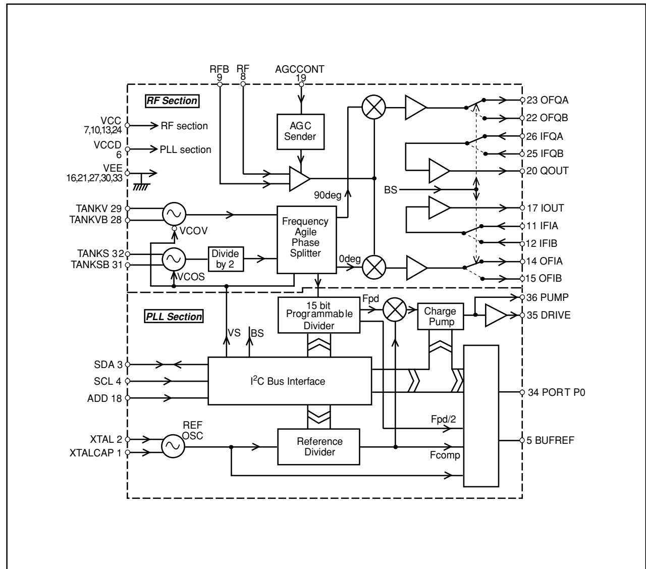
Figure 2. Block diagram
