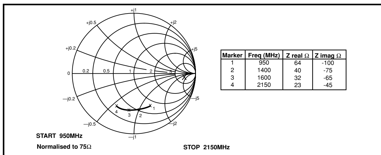
Figure 3. RF input impedance (typical)
