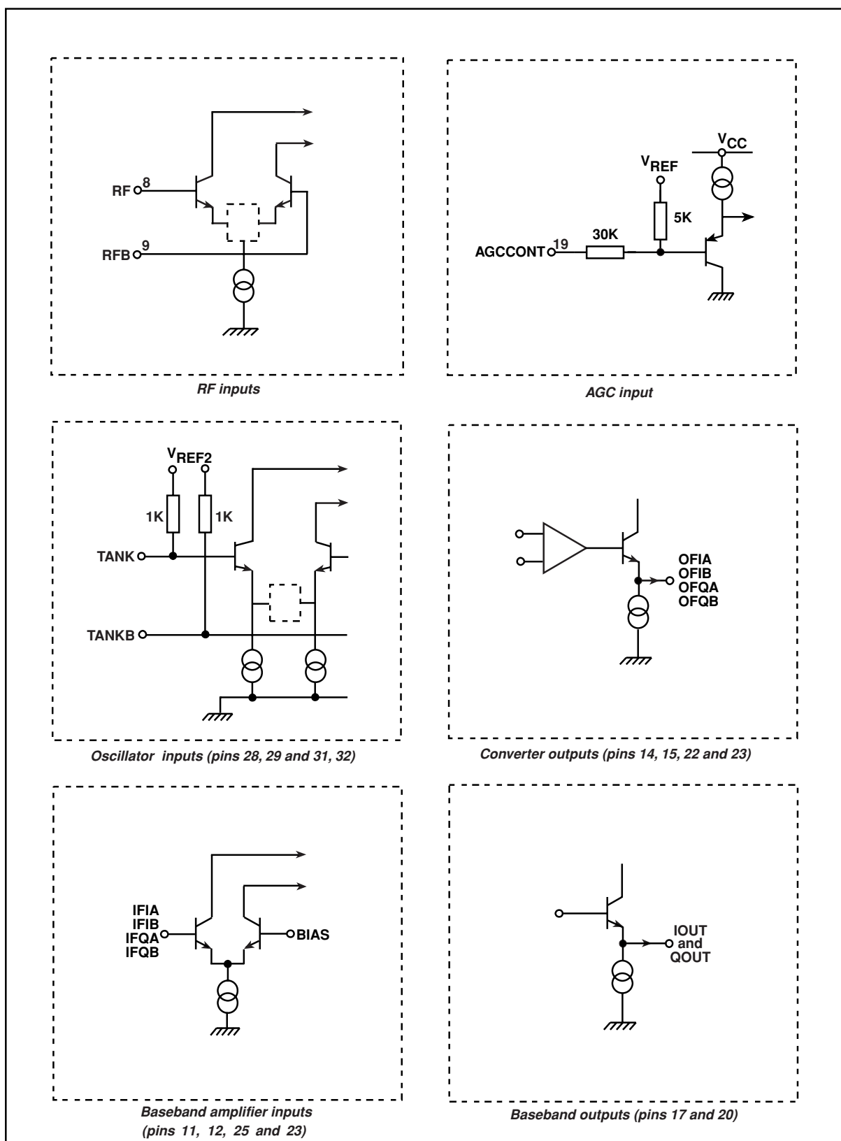
Figure 17. Input and output interface circuits (RF section)
