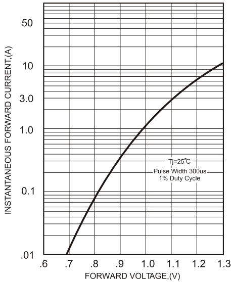
FIG.1-TYPICAL FORWARD CHARACTERISTICS
