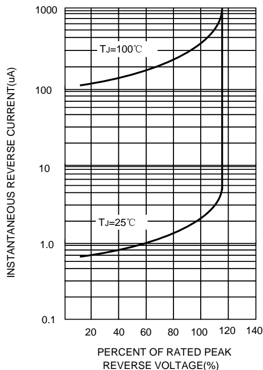
FIG.2-TYPICAL REVERSE CHARACTERISTICS
